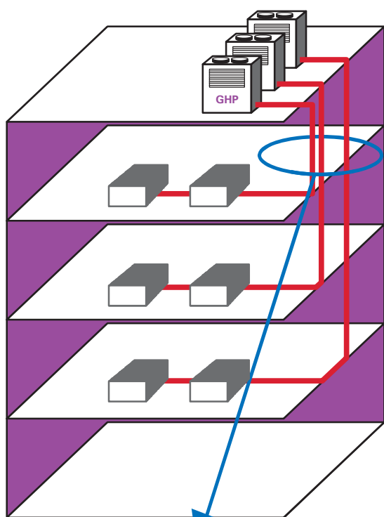
3 systems = 6 pipes
