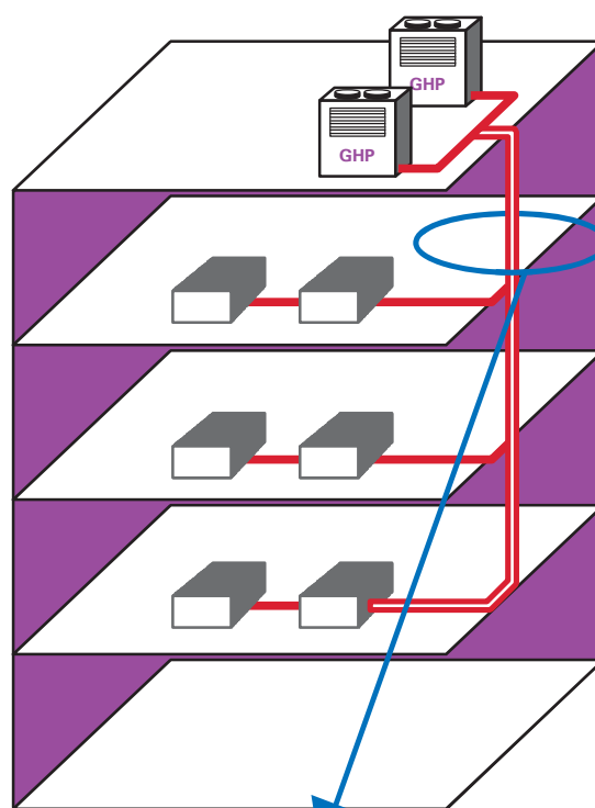
1 system = 2 pipes
